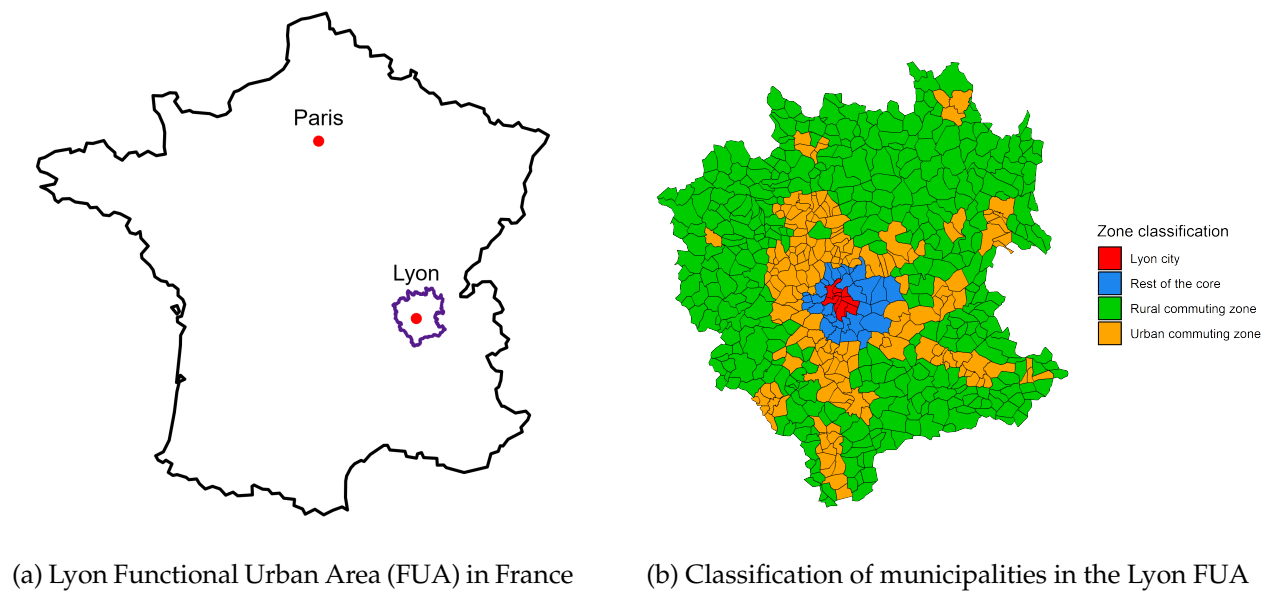
Figure 4: Maps of the Lyon Functional Urban Area and municipality classification.
