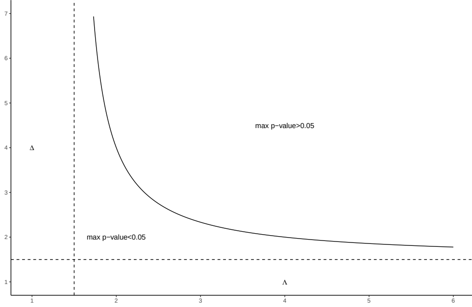
FIGURE 1 – Amplification (\Lambda, \Delta) pour \Gamma = 1.5
