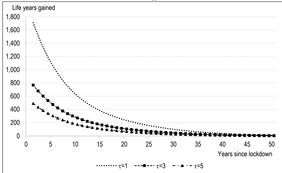
Figure III – Distribution over time of the number of life years gained (LYG) following lockdown, function of \tau (For PM_{2.5} )
